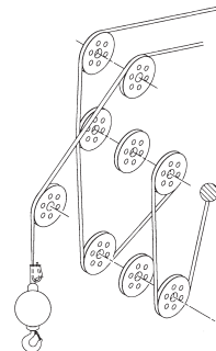
Line pulls and reeving information
