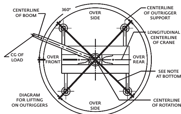
Working area diagram
